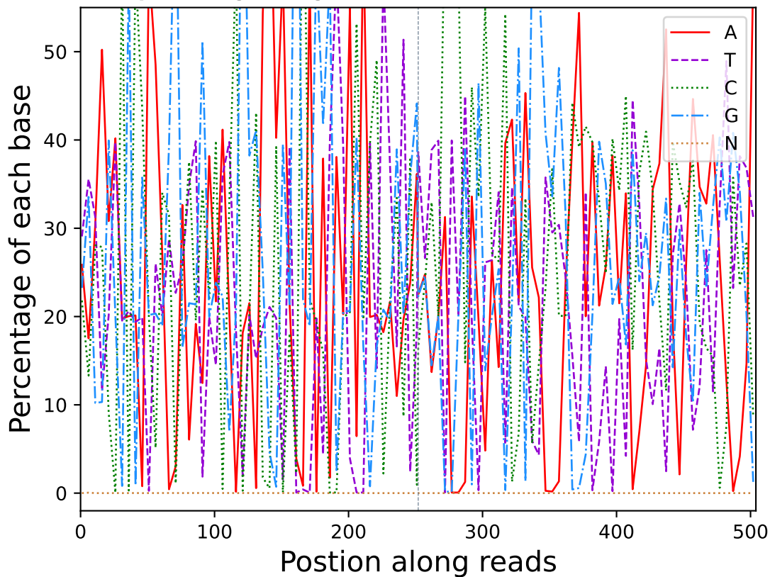
Base percentage along reads (R10812)
